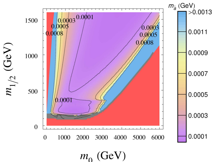
Figure 7. Contours of constant m_{\tilde{a}} in the m_0 vs. m_{1/2} plane for A_0 = 0 , \tan\beta = 10 and \mu > 0 . We assume \Omega_a h^2 = 0.11 , and \Omega_{\tilde{a}}^{\text{TP}} h^2 = 0.006 and \Omega_{\tilde{a}}^{\text{NTP}} = 6 \times 10^{-6} .
