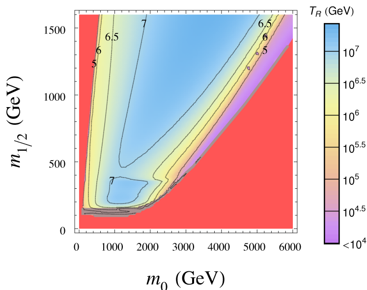
Figure 8. Contours of constant T_R in the m_0 vs. m_{1/2} plane for A_0 = 0 , \tan\beta = 30 and \mu > 0 . We assume \Omega_a h^2 = 0.11 , and \Omega_{\tilde{a}}^{\text{TP}} h^2 = 0.006 and \Omega_{\tilde{a}}^{\text{NTP}} = 6 \times 10^{-6} .
