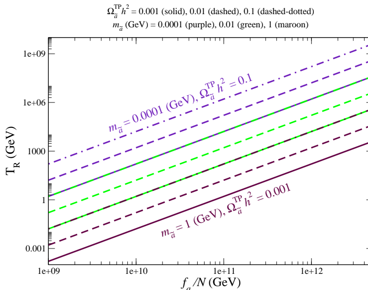
Figure 1. A plot of the expected re-heat temperature of the universe T_R versus PQ breaking scale f_a/N for \Omega_a^{\text{TP}} h^2 = 0.001 (solid), 0.01 (dashed) and 0.1 (dot-dashed), and with m_{\tilde{a}} = 10^{-4} (purple), 10^{-2} (green) and 1 GeV (maroon). (The solid purple and dot-dashed green, and also the solid green and dot-dashed maroon lines coincide.)
