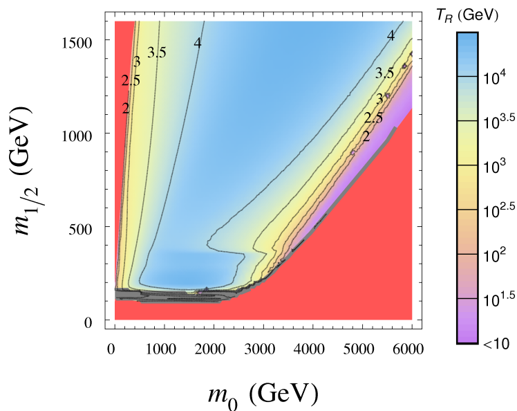
Figure 4. Contours of constant T_R in the m_0 vs. m_{1/2} plane for A_0 = 0 , \tan\beta = 10 and \mu > 0 . We assume \Omega_a h^2 = 0.11 , and \Omega_{\tilde{a}}^{\text{TP}} h^2 = \Omega_{\tilde{a}}^{\text{NTP}} = 0.003 . The lower right red region is excluded due to lack of appropriate EWSB, while the left-side red region yields a stau NLSP. The gray region is excluded by LEP2 limits on the chargino mass.
