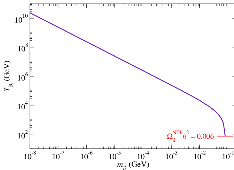
Figure 10. Plot of the value of T_R needed versus m_{\tilde{a}} for the mSUGRA point with m_0 = 1000 GeV, m_{1/2} = 300 GeV, A_0 = 0 , \tan \beta = 10 and \mu > 0 . We assume \Omega_a h^2 = 0.11 , and that \Omega_a^{\text{TP}} h^2 + \Omega_a^{\text{NTP}} = 0.006 .
