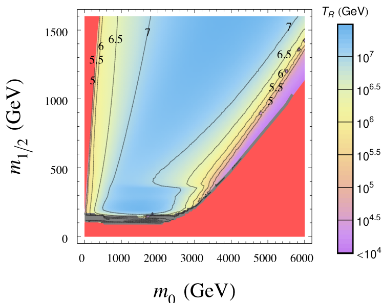
Figure 6. Contours of constant T_R in the m_0 vs. m_{1/2} plane for A_0 = 0 , \tan\beta = 10 and \mu > 0 . We assume \Omega_a h^2 = 0.11 , and \Omega_{\tilde{a}}^{\text{TP}} h^2 = 0.006 and \Omega_{\tilde{a}}^{\text{NTP}} = 6 \times 10^{-6} .
