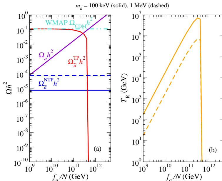
Figure 3. Axion and TP and NTP axino contributions to dark matter density for m_{\tilde{a}} = 100 keV versus PQ breaking scale f_a/N .
