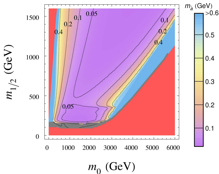
Figure 5. Contours of constant m_{\tilde{a}} in the m_0 vs. m_{1/2} plane for A_0 = 0 , \tan\beta = 10 and \mu > 0 . We assume \Omega_a h^2 = 0.11 , and \Omega_{\tilde{a}}^{\text{TP}} h^2 = \Omega_{\tilde{a}}^{\text{NTP}} = 0.003 .
